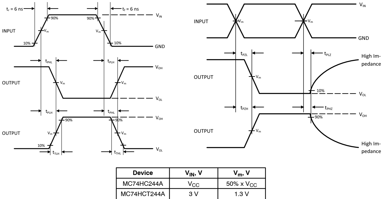
Figure 2. Switching Waveforms
