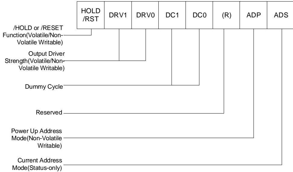
Figure 4c. Status Register-3
