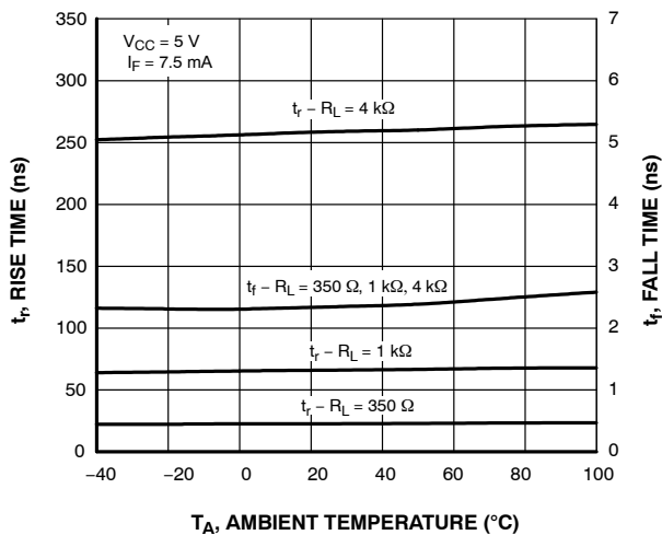
Figure 21. Rise and Fall Times vs. Ambient Temperature
