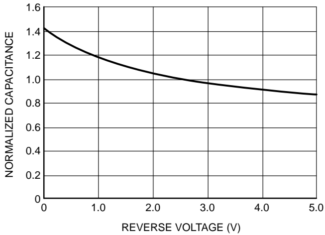
Figure 3. Typical Capacitance
