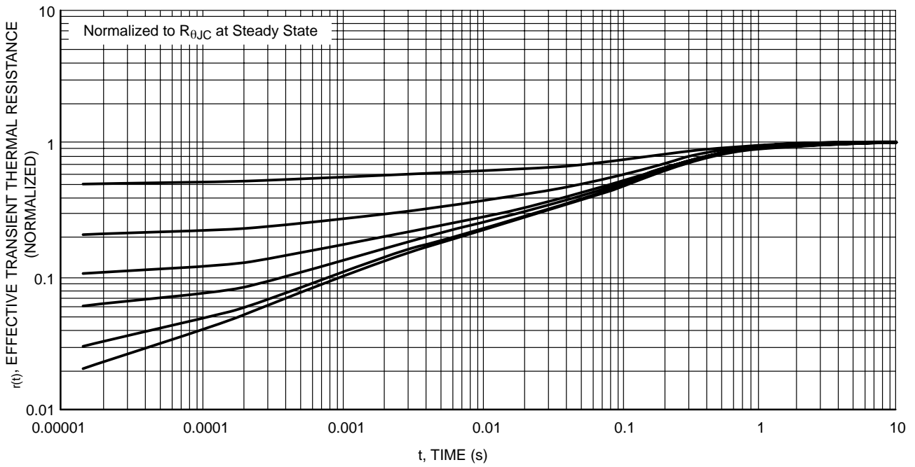
Figure 12. Thermal Response
