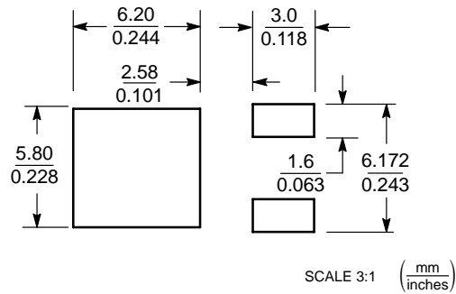
Figure 13. DPAK
