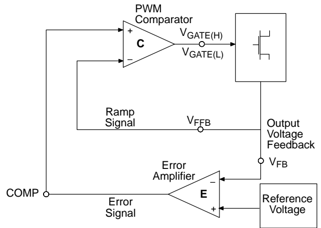
Figure 1. V 2 Control Diagram
