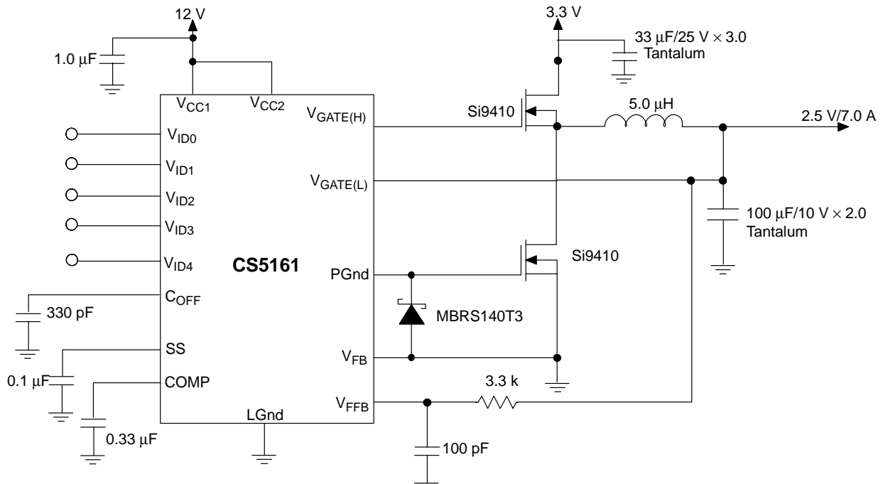
Figure 23. 3.3 V to 2.5 V/7.0 A Converter with 12 V Bias.
