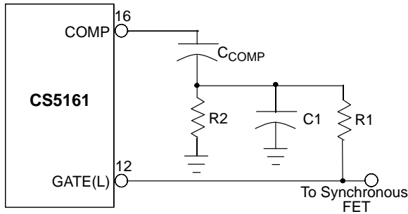
Figure 17. Small RC Filter Provides the Proper Voltage Ramp at the Beginning of each On-Time Cycle
