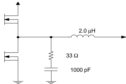
Figure 19. Filter Components
