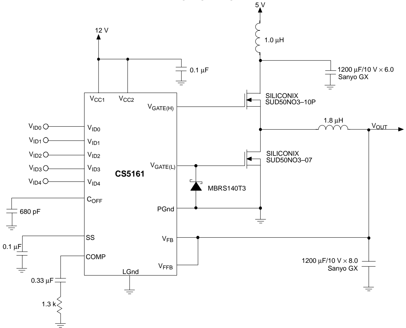
5.0 V to 1.5 V/15 A Core Logic Converter with 12 V Bias
