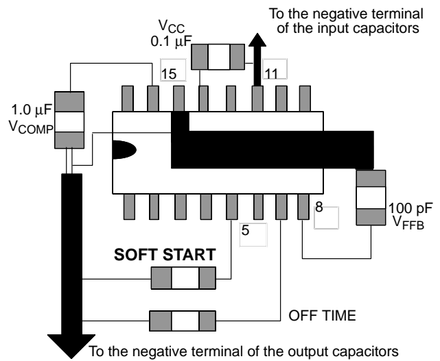
Figure 21. Layout Guidelines
