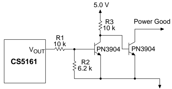
Figure 15. Implementing Power Good with the CS5161/5161H
