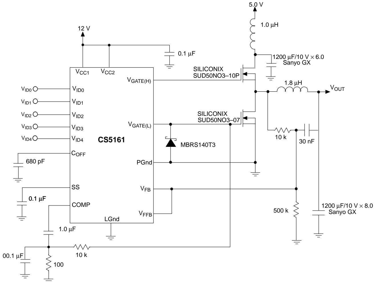
Figure 24. Pentium ® III Converter with Slope Compensation and Adaptive Voltage Positioning
