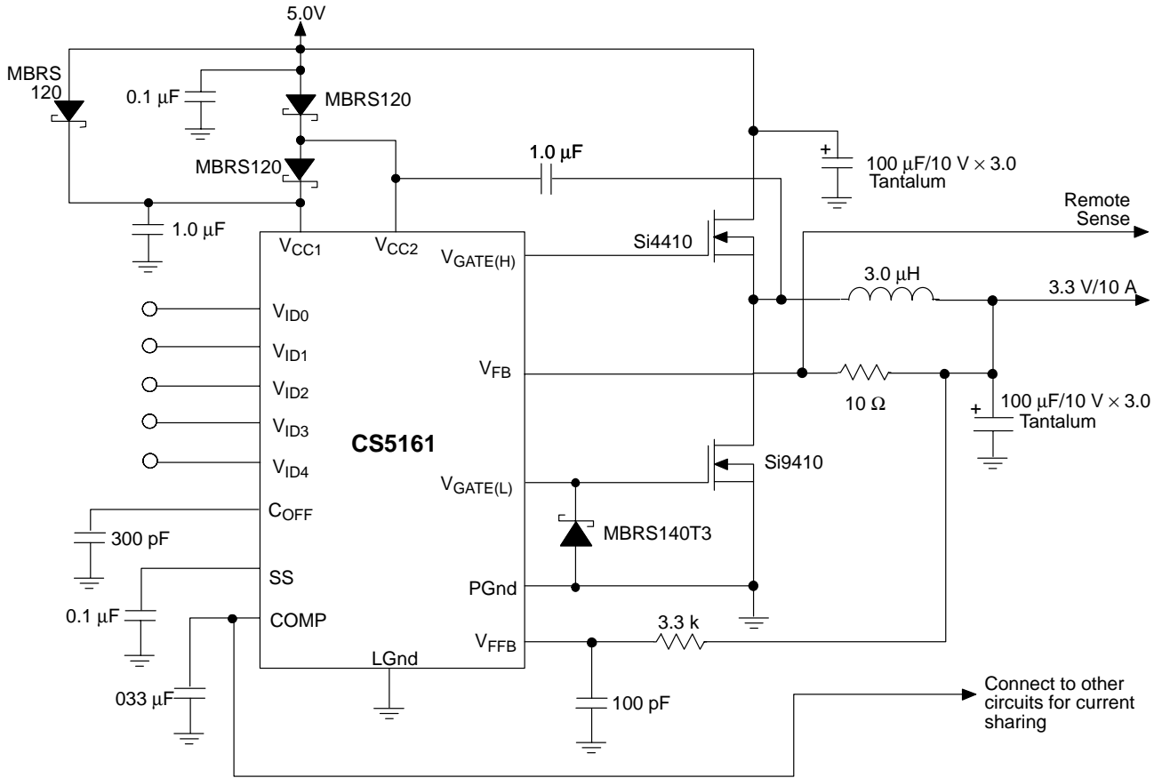
Figure 22. 12 V to 3.3 V/10 A Converter with Remote Sense and Current Sharing
