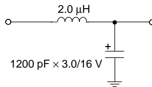
Figure 20. Input Filter
