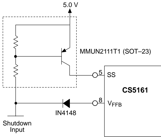
Figure 14. Implementing Shutdown with the CS5161/5161H
