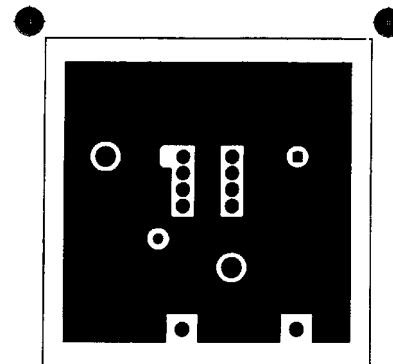
TOP LAYOUT
