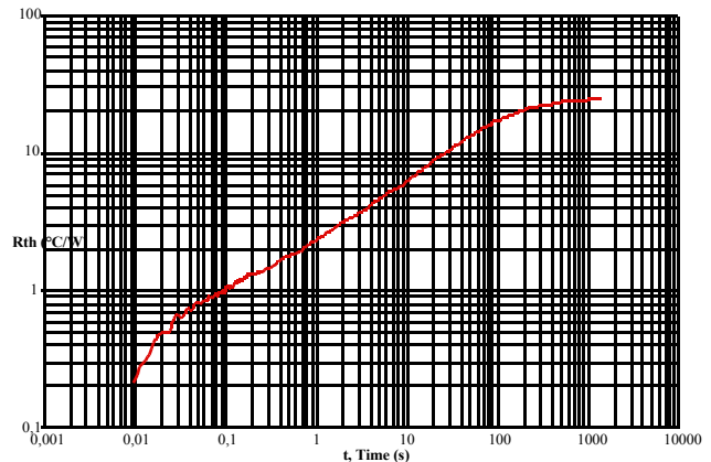
Figure 20. 33887 Thermal Response
