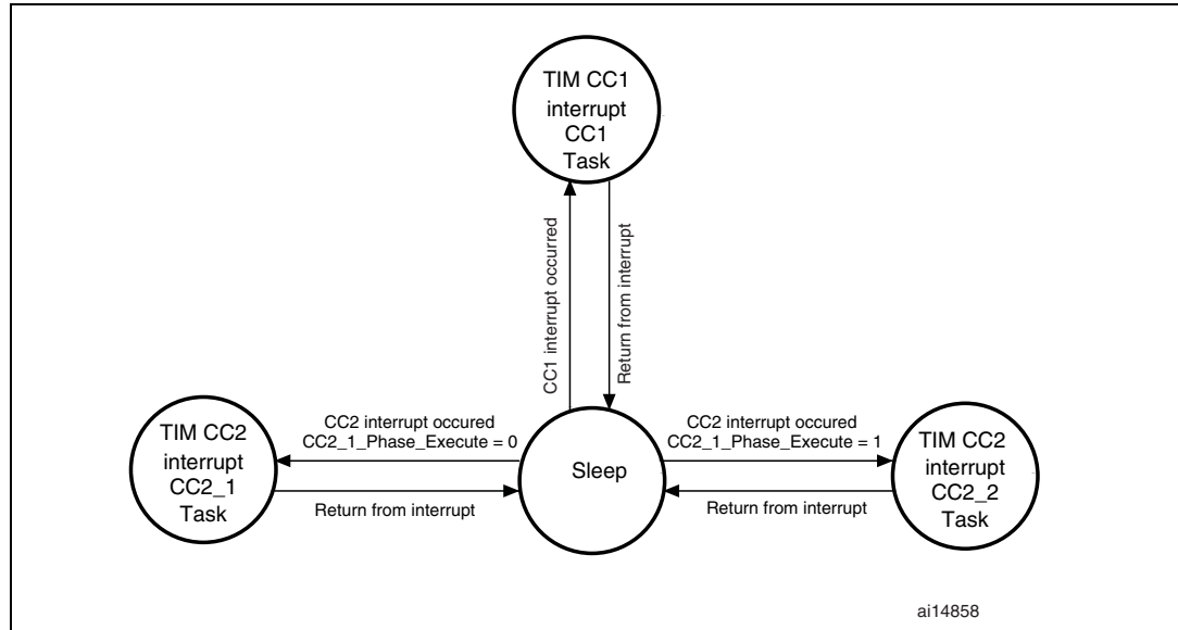
Figure 17. Timer method state machine
