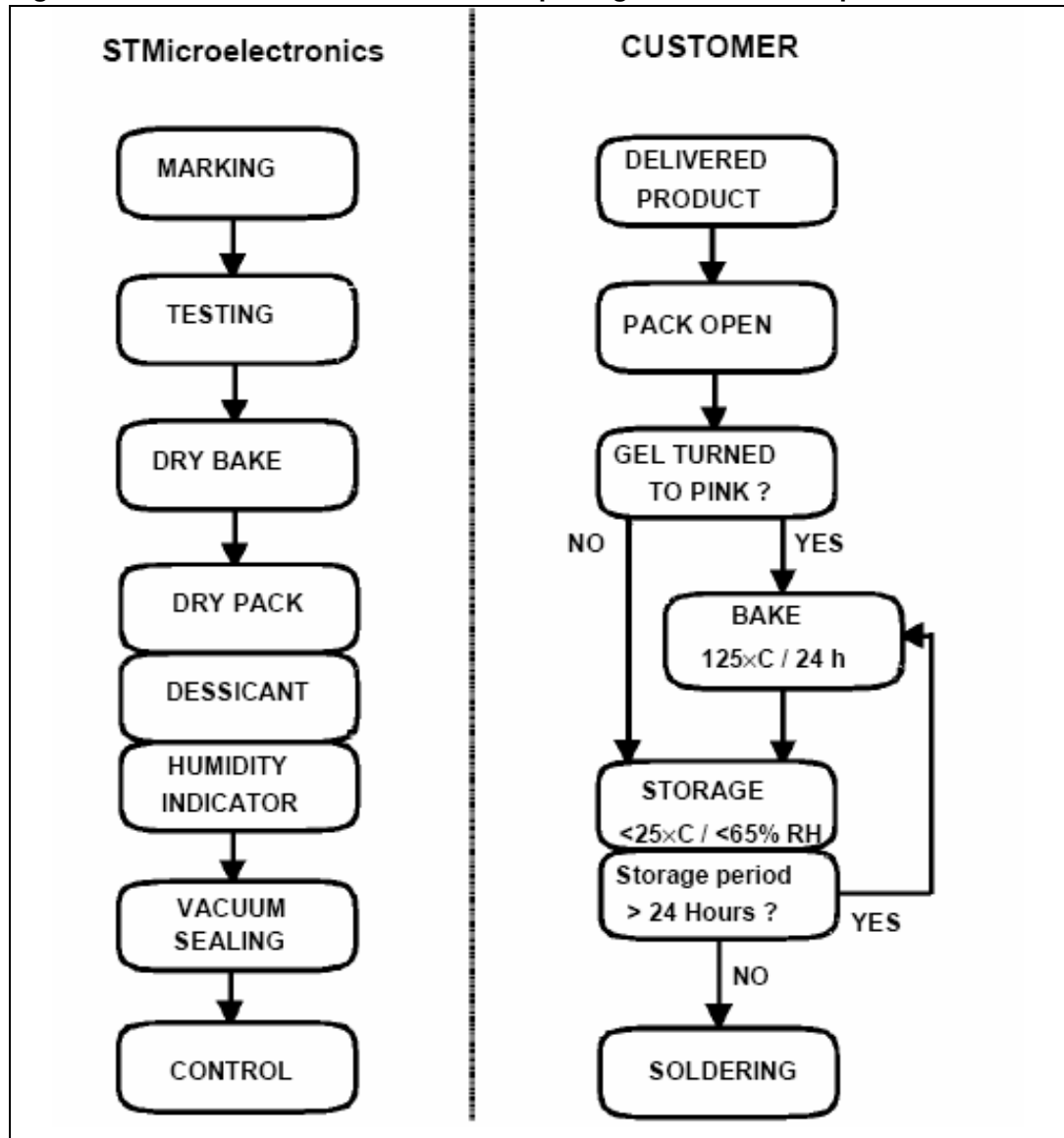
Figure 6. Recommended flow to control package moisture absorption
