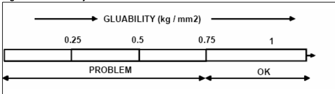
Figure 5. Gluability evaluation with a shear test
