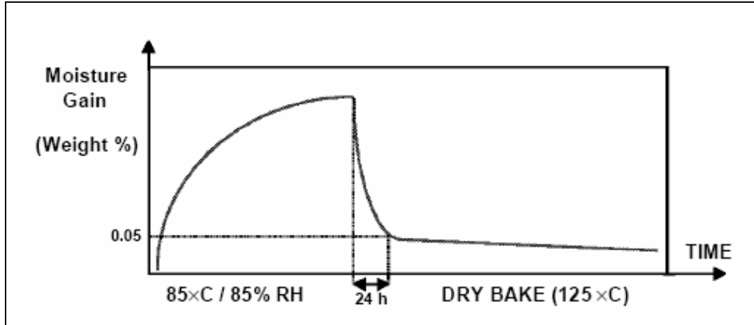
Figure 7. Moisture absorption / drying curve.
